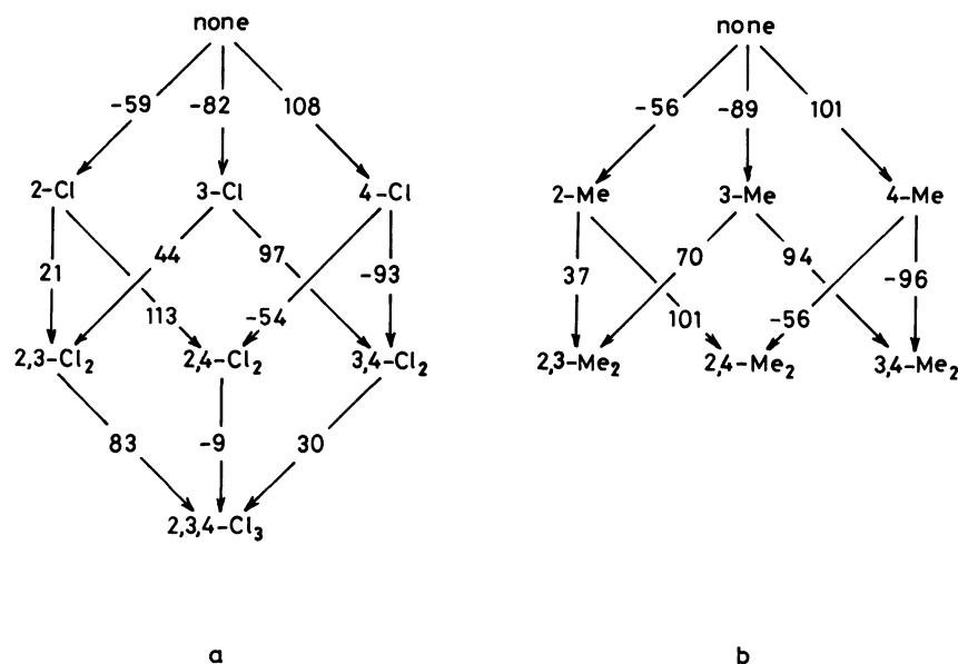
Fig. 1. The change in the clearing point (°C) of N -[4-(4-methoxybenzoyloxy)benzylidene]aniline by (a) chloro and (b) methyl substitution.
